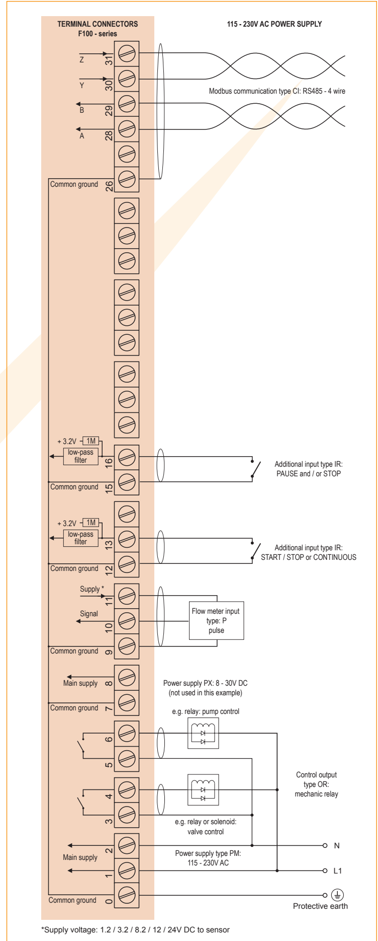
Typical wiring diagram F133-P-CI-OR-PM
