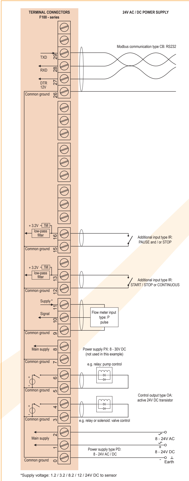
Typical wiring diagram F133-P-CB-OA-PD
