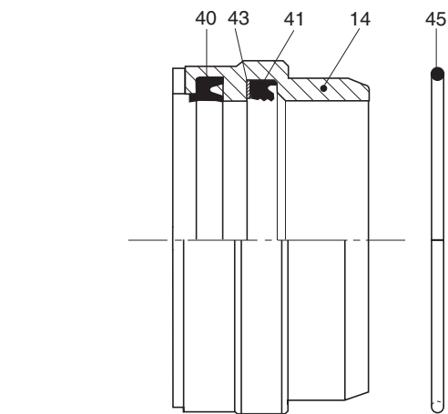
Bushing and Seals
