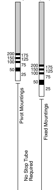
Recommended Length of Stop Tube (mm)
