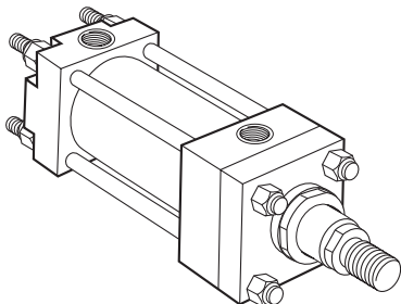
Model 52 Tie Rods Extended Cap End (ISO Style MX2)
