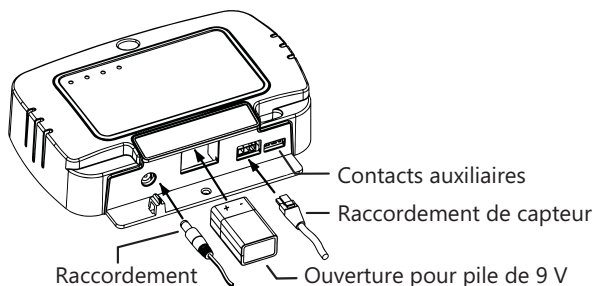
Figure 1. Emplacements de raccordement
