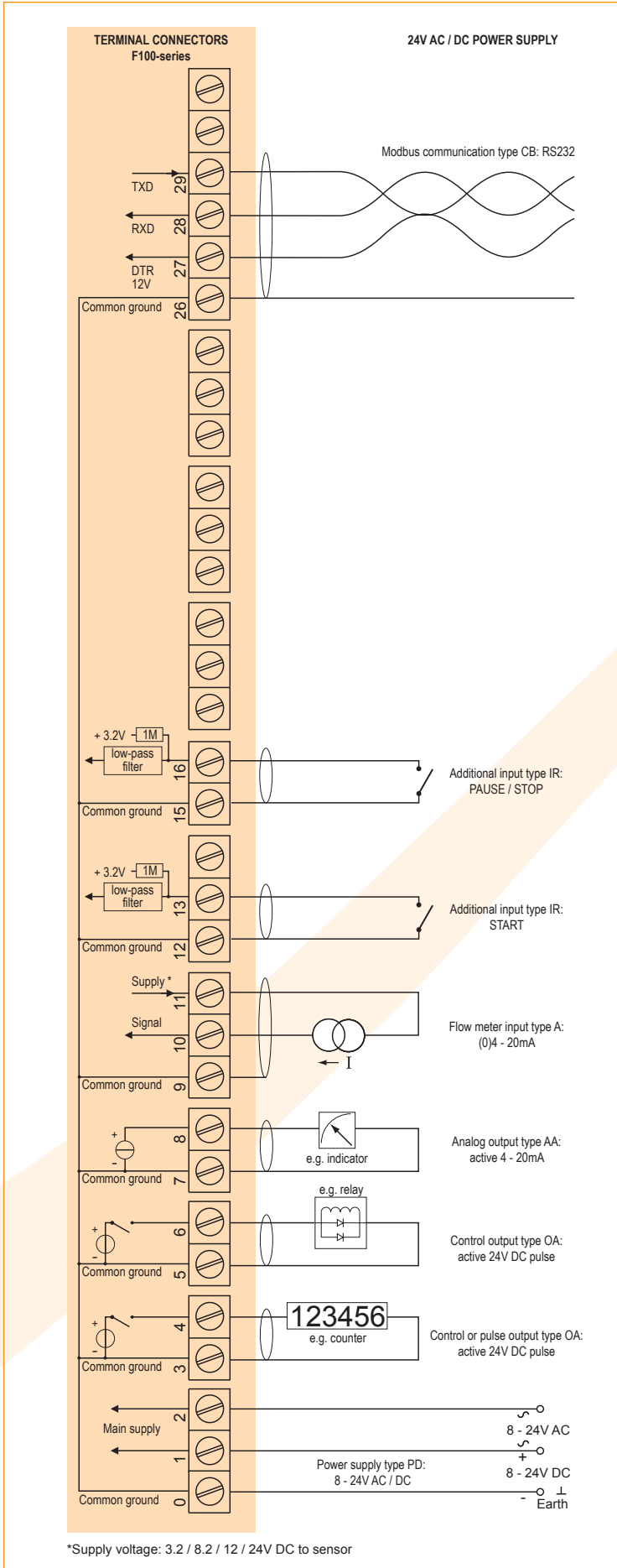
Typical wiring diagram F131-A-AA-CB-OA-PD
