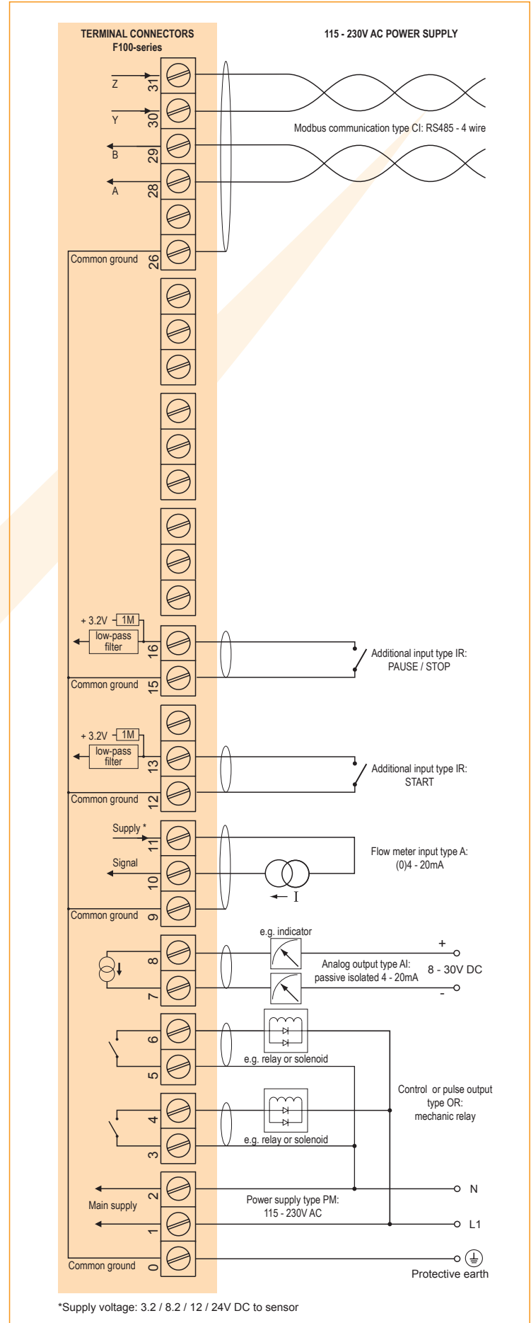
Typical wiring diagram F131-A-AI-CI-OR-PM
