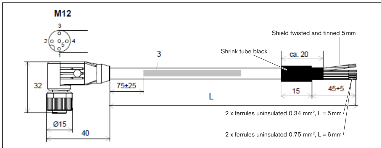
Figure 6: Example M12 connection cable, length 70 cm
