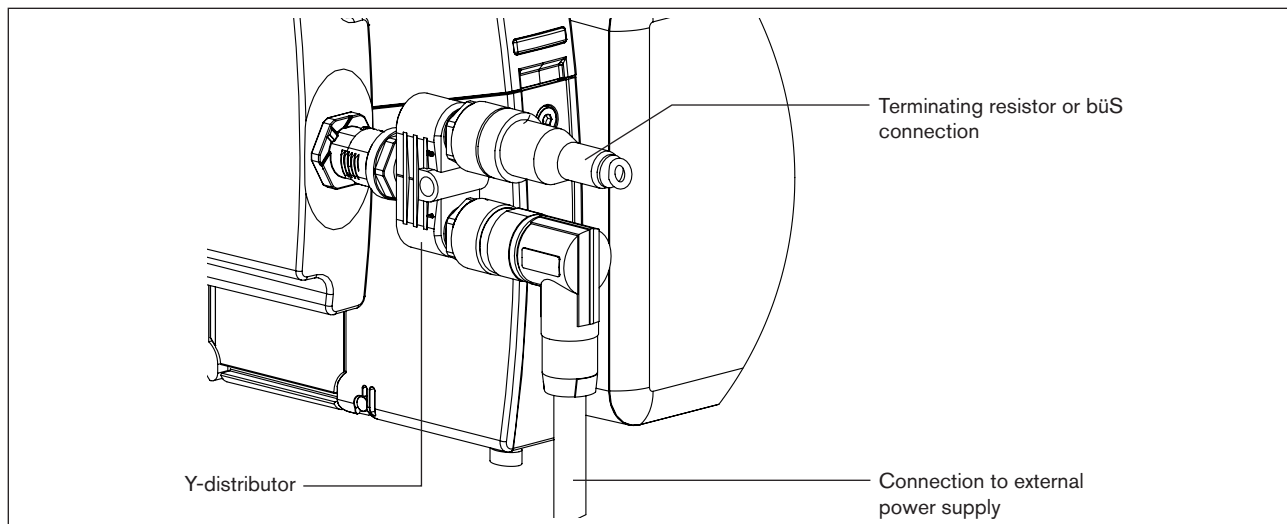
Figure 7: Example electrical connection with Y-distributor
